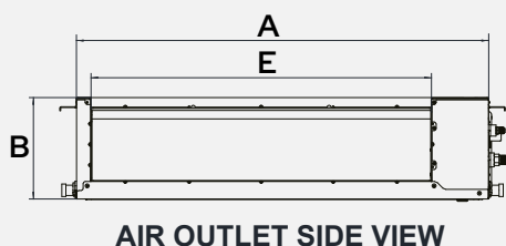
AIR OUTLET SIDE VIEW
